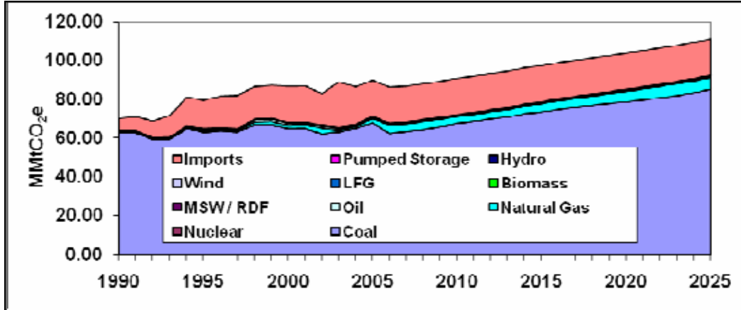
Figure 3-1. Recent and projected GHG emissions from the electricity sector, Michigan, 2005–2025 (consumption basis)
